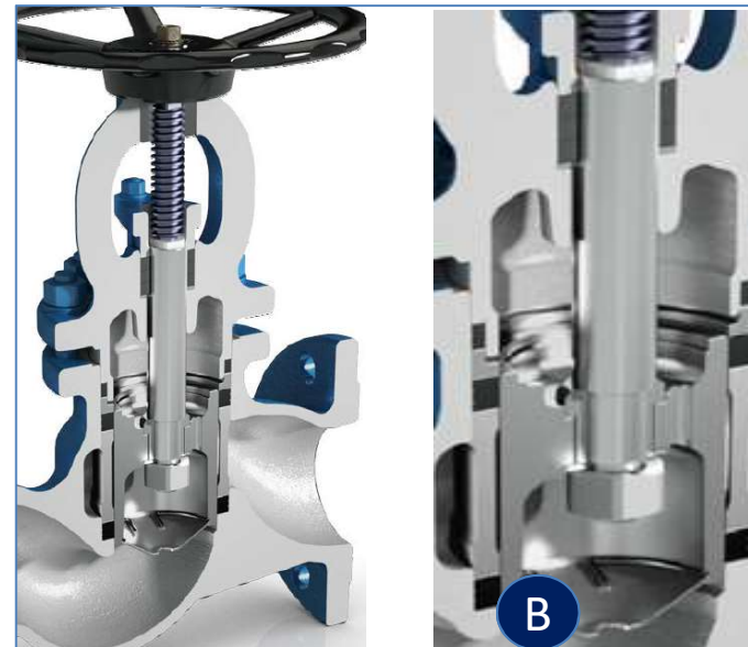
DN65 – 200 pressure balanced
